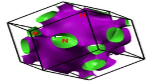
Fermi Surface of LaRu_4P_{12}
