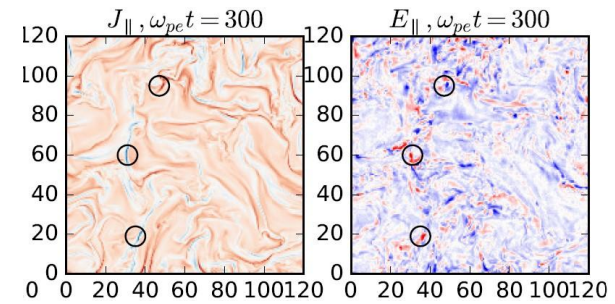
Plasma Turbulence
