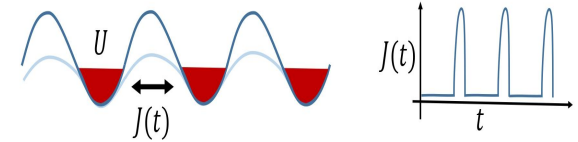
Bosonic Josephson junctions
