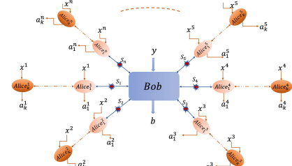
Device-independent nonlocal correlation in Star-network
