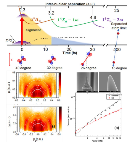
Atomic and Molecular Dynamics
