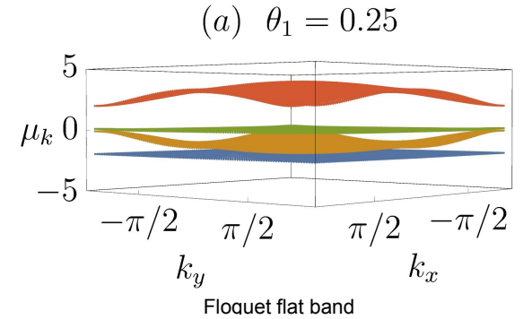
Floquet flat band
